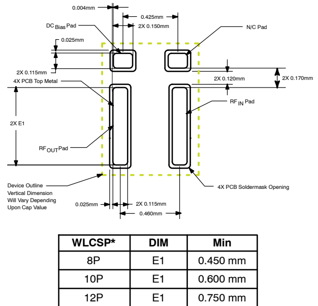
Figure 8. Recommended Pad Layout
