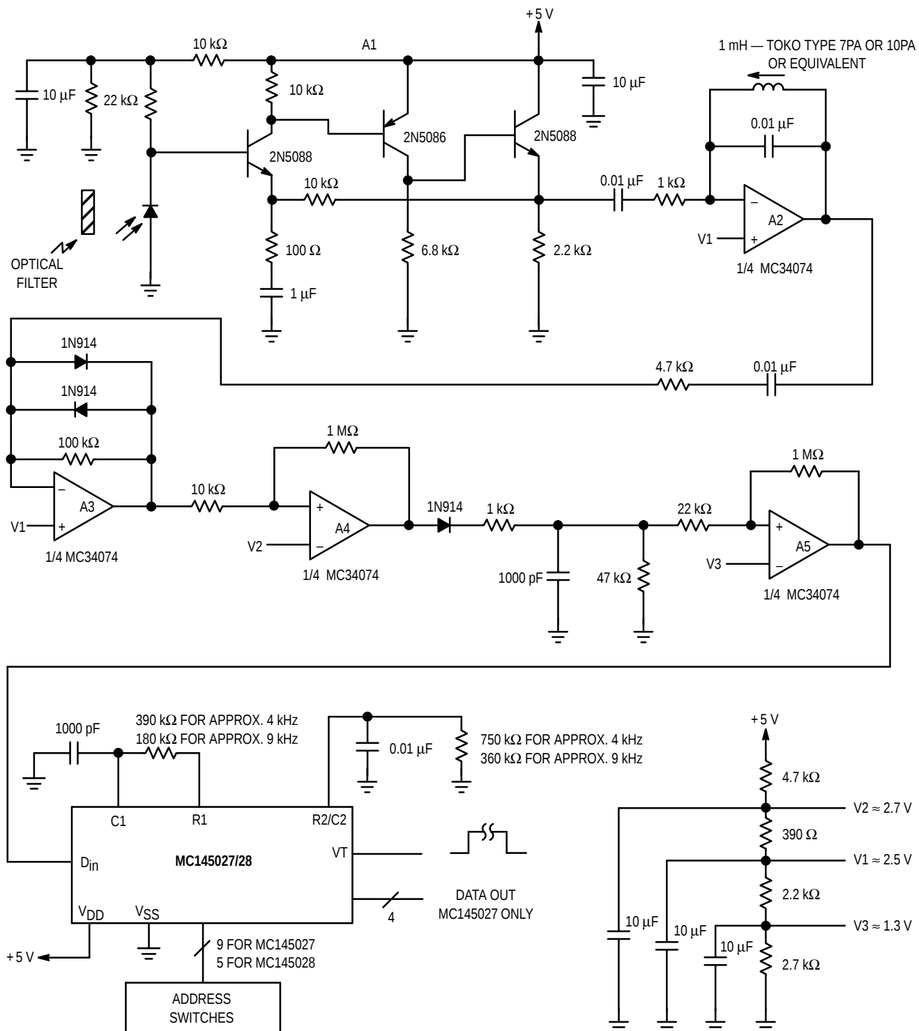
Figure 20. Infrared Receiver
