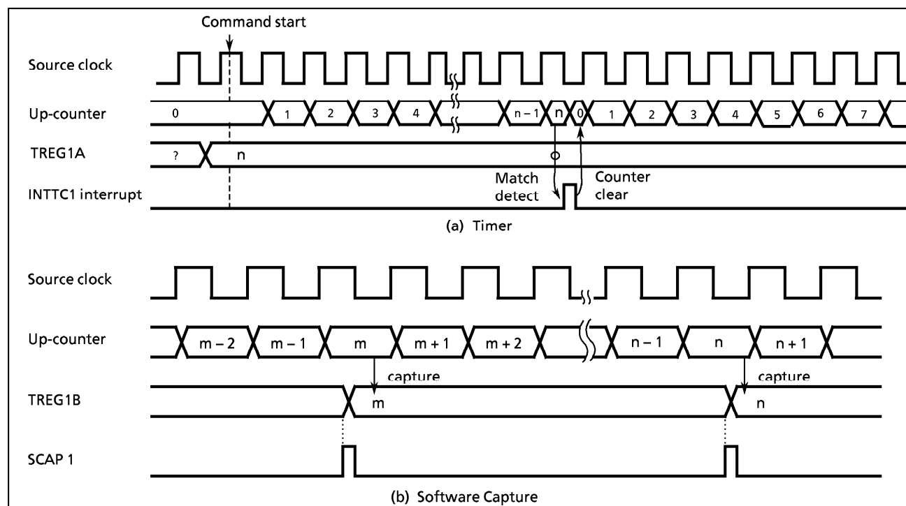
Figure 2-18. Timer Mode Timing Chart
