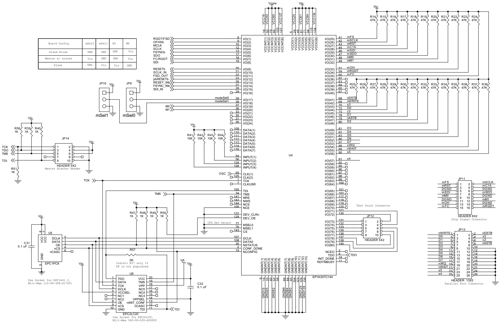
Figure 20. Si30xx Motherboard Schematic (3 of 3)
