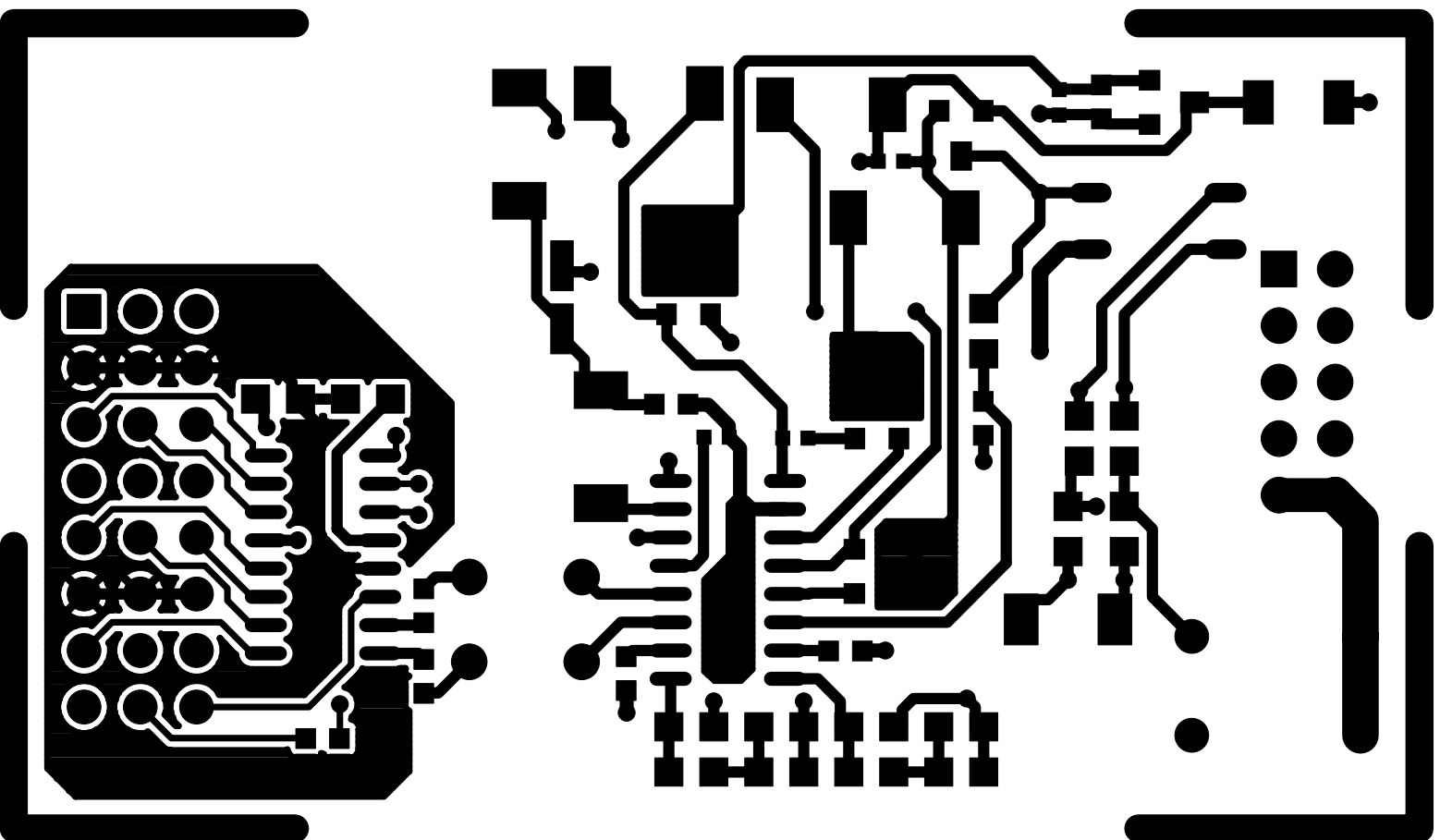
Figure 16. Si3056 Daughter Card Component Layer
