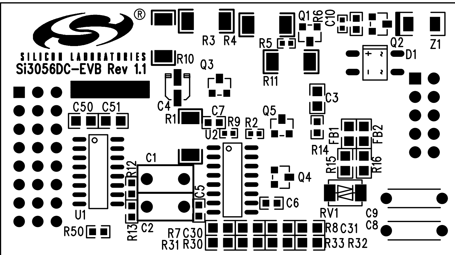
Figure 15. Si3056 Daughter Card Silkscreen
