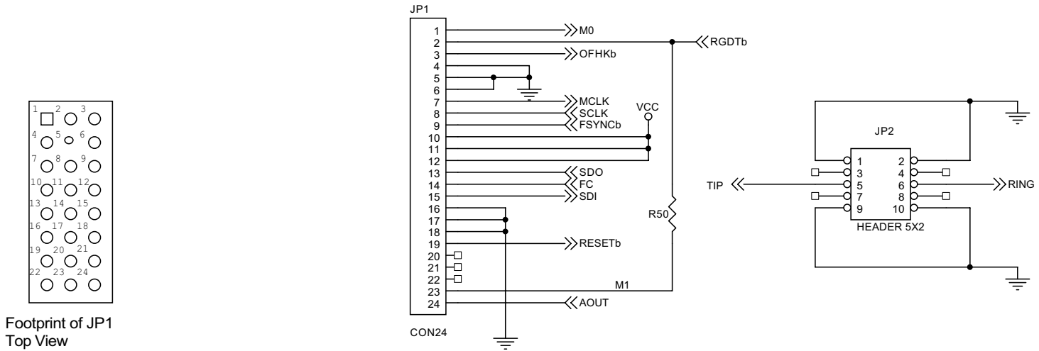
Figure 12. Si3034/35/44 Daughter Card Schematic (2 of 2)
