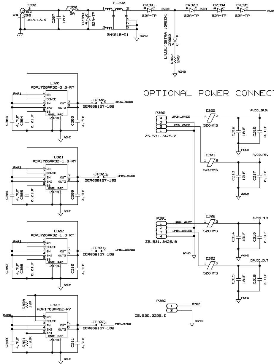
Figure 17. Board Power Supply Circuits
