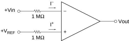
Figure 7 Positive Input Voltage Comparator
