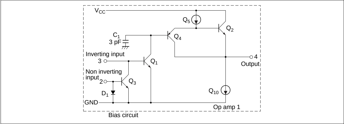
Figure 1 HA17301 Internal Equivalent Circuit
