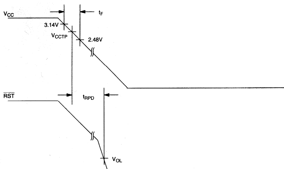
POWER-DOWN Figure 5
