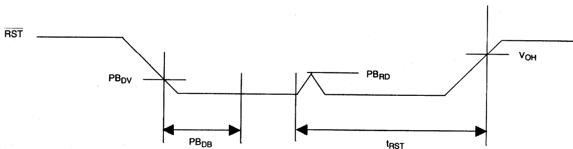
POWER-UP Figure 4
