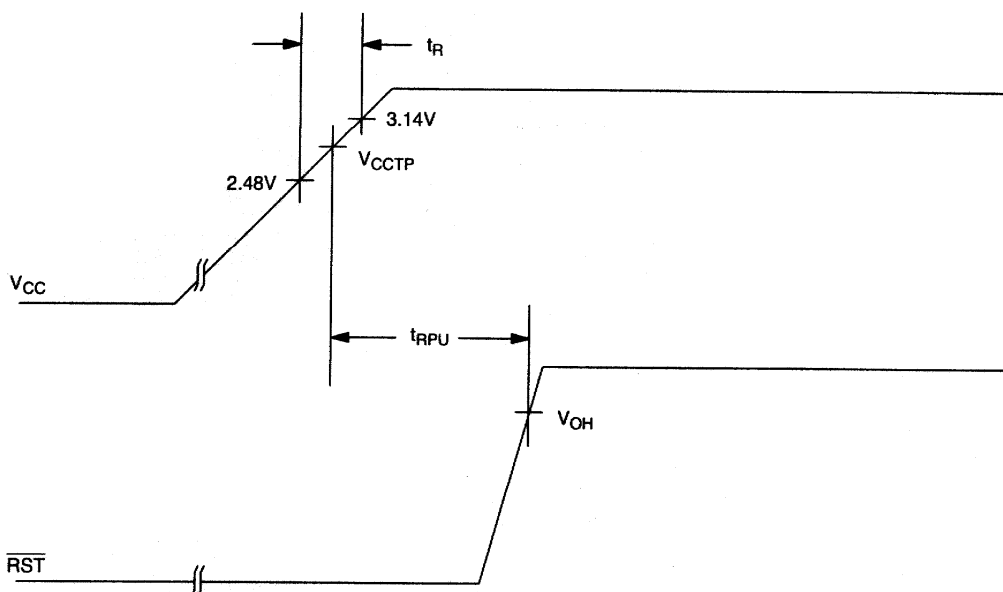
POWER-UP Figure 4
