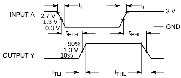
Figure 3. Switching Waveforms
