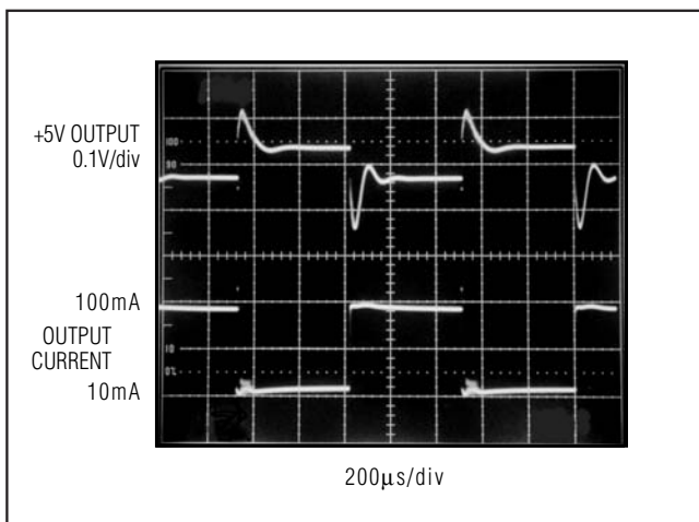
Figure 12. Output Response to 10mA/100mA Load Step with 10μF Output Capacitor (1.5Ω ESR)
