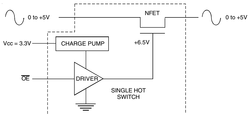
Rail-to-Rail Switching
