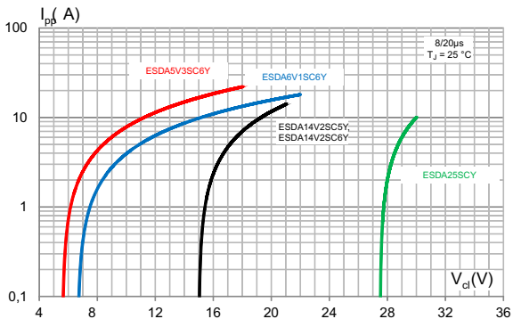
Figure 5. Clamping voltage versus peak pulse current (typical values, 8/20 \mu\text{s} waveform)
