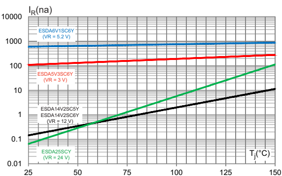
Figure 6. Leakage current versus junction temperature (typical values)
