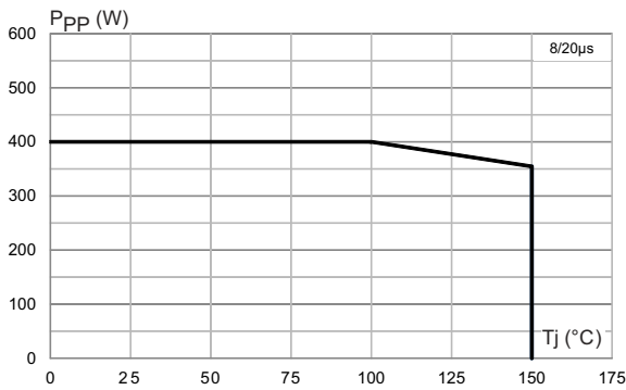
Figure 3. Pulse power versus junction temperature
