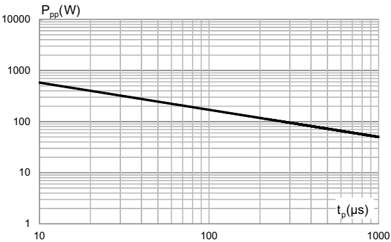
Figure 4. Peak pulse power versus exponential pulse duration (typical values)
