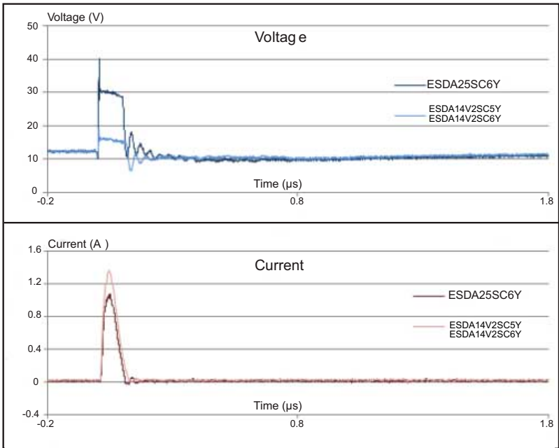
Figure 10. ISO7637-2 pulse 3b response ( V_S = 100\text{ V} )
