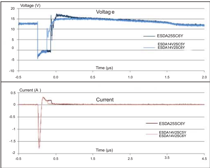
Figure 9. ISO7637-2 pulse 3a response ( V_S = -150\text{ V} )
