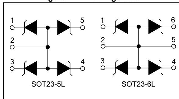
Figure 1. Pin configuration
