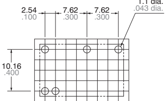
2 coil latching
