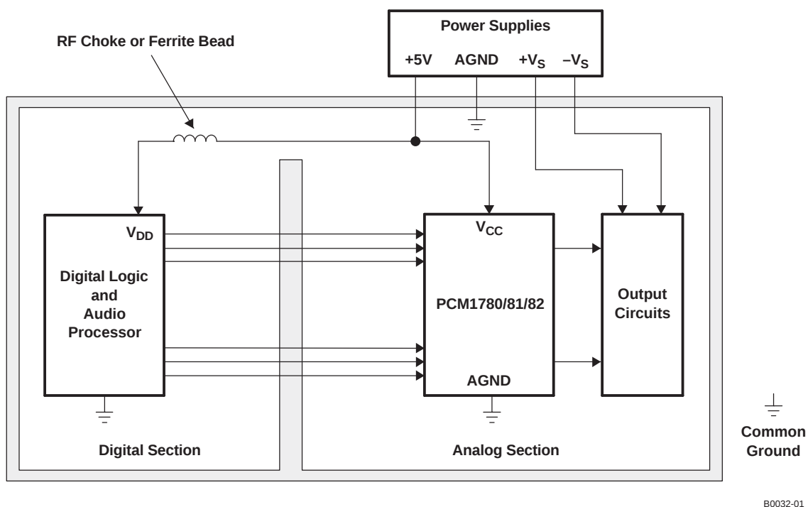
Figure 31. Single-Supply PCB Layout
