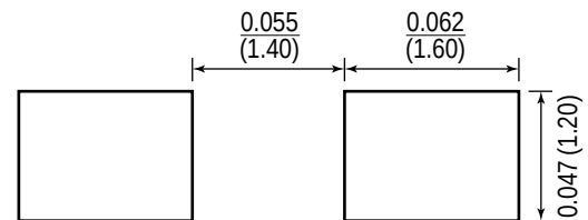
Mounting Pad Layout
