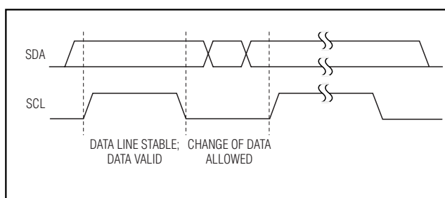
Figure 10. Bit Transfer
