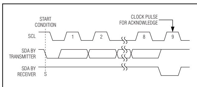
Figure 11. Acknowledge
