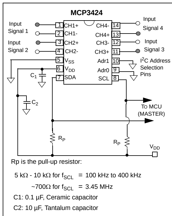
FIGURE 6-1: Typical Connection.
