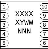
10-Lead DFN (3x3) (MCP3423)
