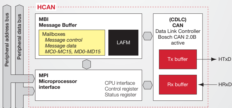
HCAN Block Diagram
