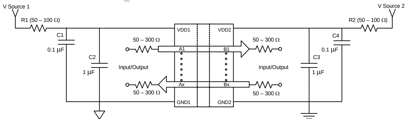
Figure 8. Recommended Bypass Components for the Si84xx Digital Isolator Family
