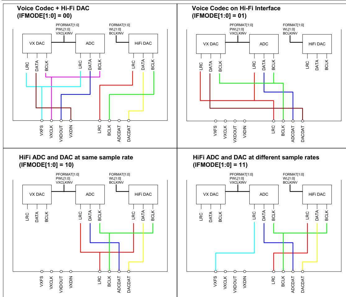
Figure 23 Audio Interface Configuration
