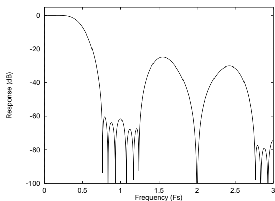
Figure 34 AC Digital Filter Frequency Response – Type 3
