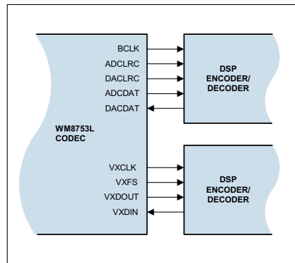
Figure 15a Master Mode
