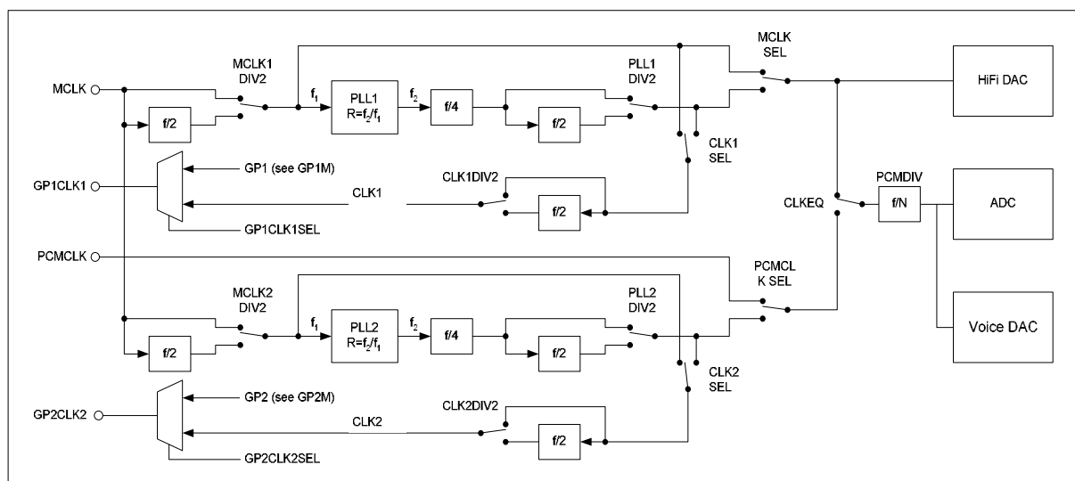
Figure 26 PLL and Clock Select Circuit
