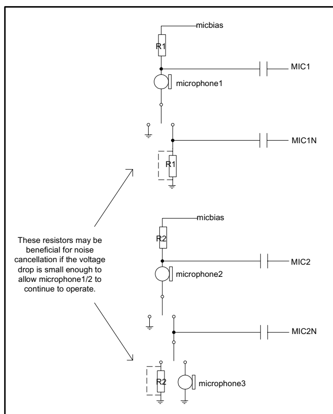
Figure 7 Suggested External Microphone Input Configuration
