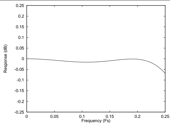
Figure 35 AC Digital Filter Ripple – Type 3
