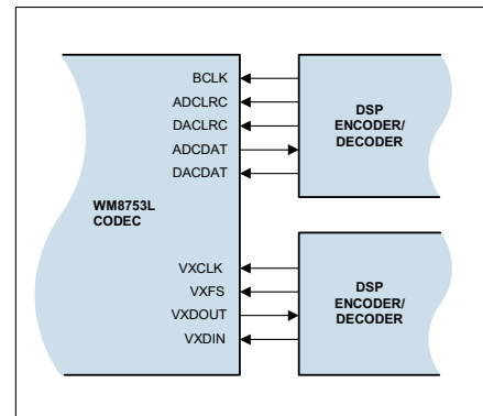
Figure 15b Slave Mode
