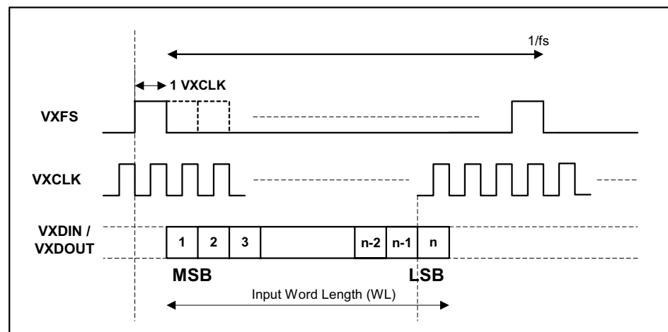
Figure 21 PCM Interface Mono Mode (mode A, PLRP=0)
