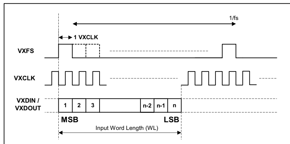
Figure 22 PCM Interface Mono Mode (mode B, PLRP=0)
