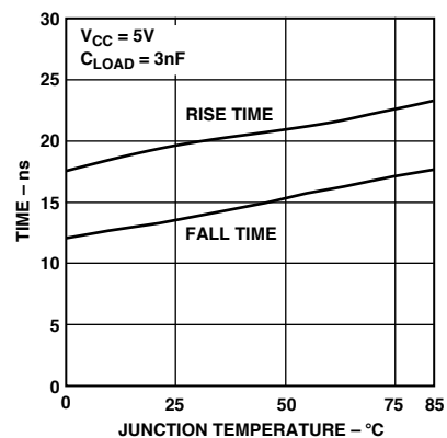
TPC 3. DRVH Rise and Fall Times vs. Temperature
