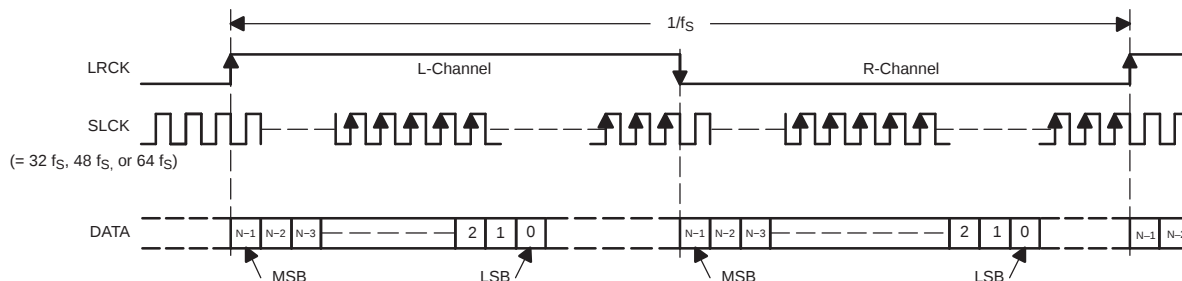
Figure 27. Left-Justified Format
