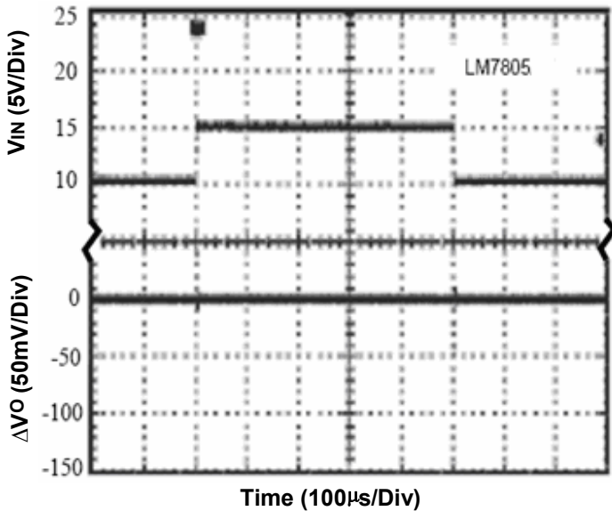
Fig.5- Line Transient (Conditions: I_o=500\text{mA} , C_o=0.1\mu\text{F} )
