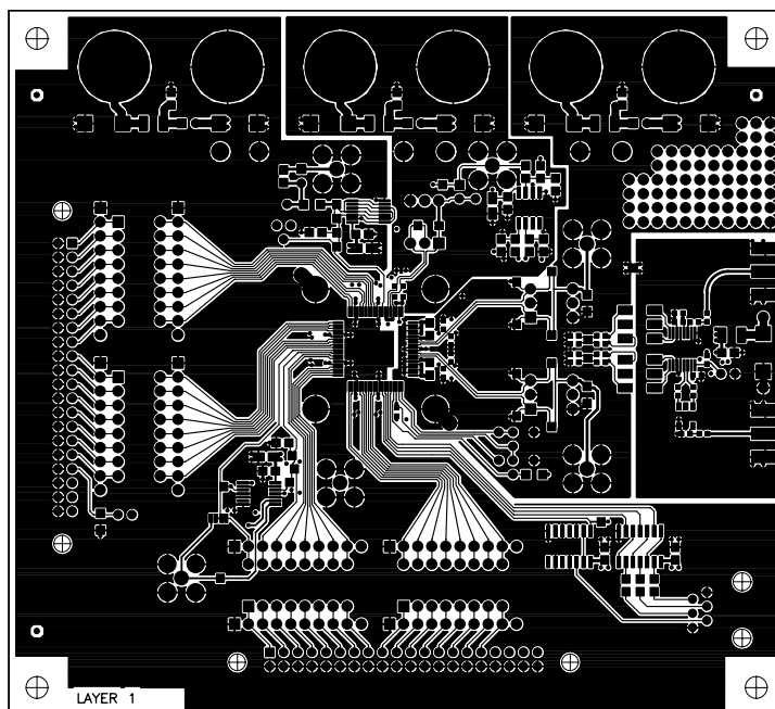
Figure 66. AD9777 Evaluation Board Layout, Layer One (Top)
