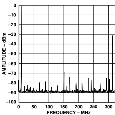
TPC 23. Single-Tone Spurious Performance, f_{OUT} = 10 MHz, f_{DATA} = 80 MSPS, Interpolation = 4×
