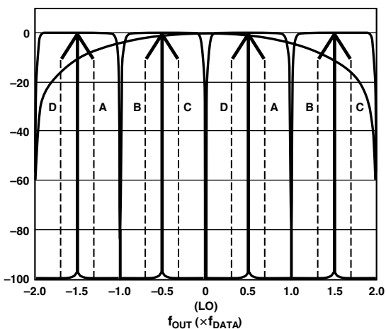
Figure 38. 2× Interpolation, Complex f_{DAC}/4 Modulation
