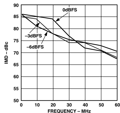
TPC 12. Third Order IMD Products vs. Two-Tone f_{OUT} @ f_{DATA} = 160 MSPS
