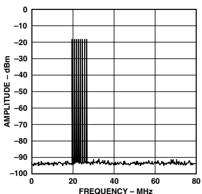
TPC 26. Eight-Tone IMD Performance, f_{DATA} = 160 MSPS, Interpolation = 8×
