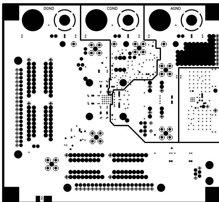
Figure 67. AD9777 Evaluation Board Layout, Layer Two (Ground Plane)
