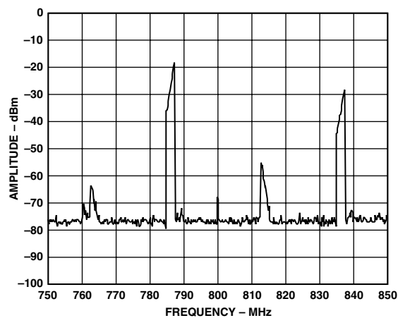
Figure 50. AD9777, Real DAC Output of Complex Input Signal Near Baseband (Positive Frequencies Only), Interpolation = 8\times , Complex Modulation in AD9777 = +f_{DAC}/8
