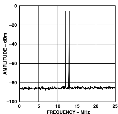
TPC 24. Two-Tone IMD Performance, f_{OUT} = 10 MHz, f_{DATA} = 50 MSPS, Interpolation = 8×
