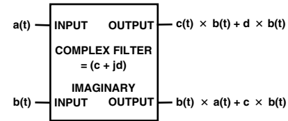
Figure 31. Realization of a Complex System
