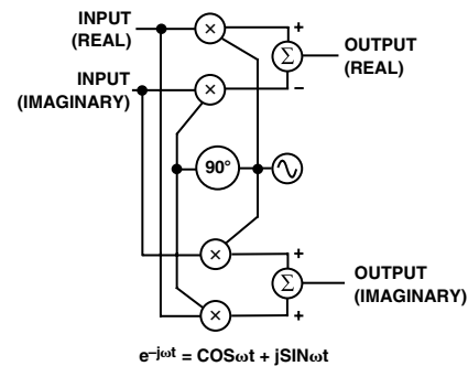
Figure 32. Implementation of a Complex Modulator
