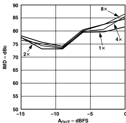
TPC 14. Third Order IMD Products vs. Two-Tone A_{OUT} and Interpolation Rate f_{DATA} = 50 MSPS for All Cases
