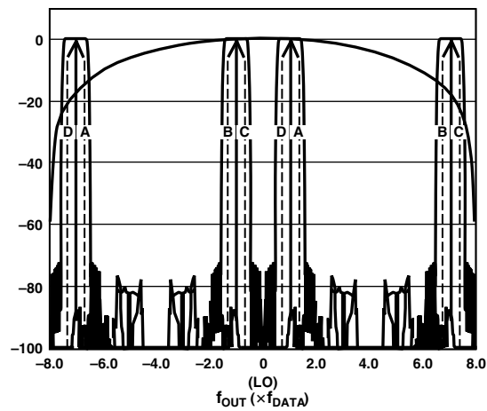
Figure 43. 8× Interpolation, Complex f_{DAC}/8 Modulation
