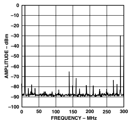
TPC 21. Single-Tone Spurious Performance, f_{OUT} = 10 MHz, f_{DATA} = 150 MSPS, Interpolation = 2×
