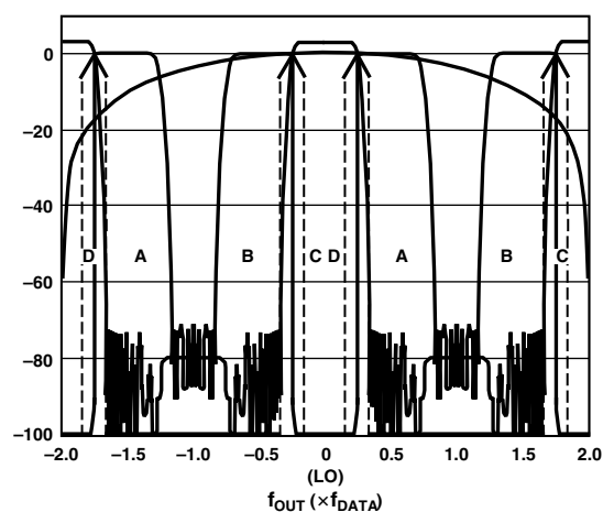
Figure 41. 2× Interpolation, Complex f_{DAC}/8 Modulation
