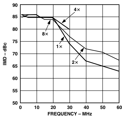
TPC 13. Third Order IMD Products vs. Two-Tone f_{OUT} and Interpolation Rate
