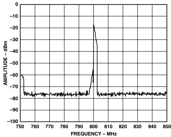
Figure 45. AD9777 Complex Output from Figure 44, Now Quadrature Modulated by AD8345 (LO = 800 MHz)
