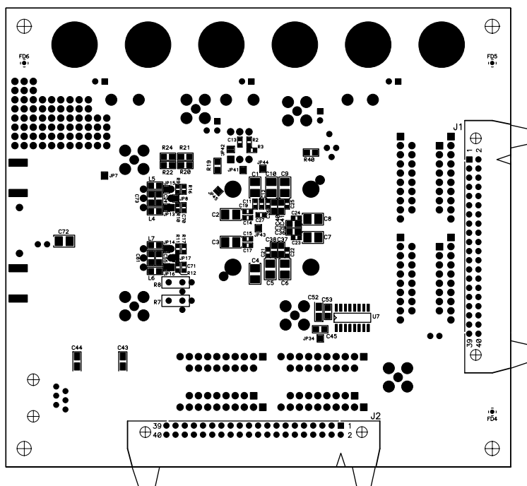
Figure 65. AD9777 Evaluation Board Components, Bottom Side
