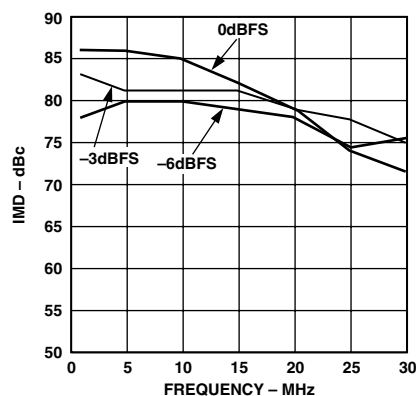
TPC 11. Third Order IMD Products vs. Two-Tone f_{OUT} @ f_{DATA} = 78 MSPS
