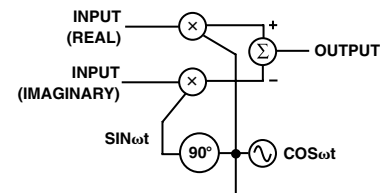
Figure 33. Quadrature Modulator
