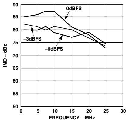
TPC 10. Third Order IMD Products vs. Two-Tone f_{OUT} @ f_{DATA} = 65 MSPS
