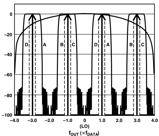
Figure 39. 4× Interpolation, Complex f_{DAC}/4 Modulation
