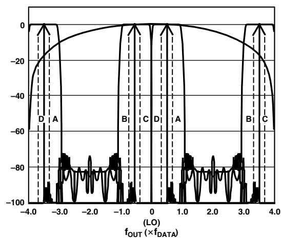
Figure 42. 4× Interpolation, Complex f_{DAC}/8 Modulation
