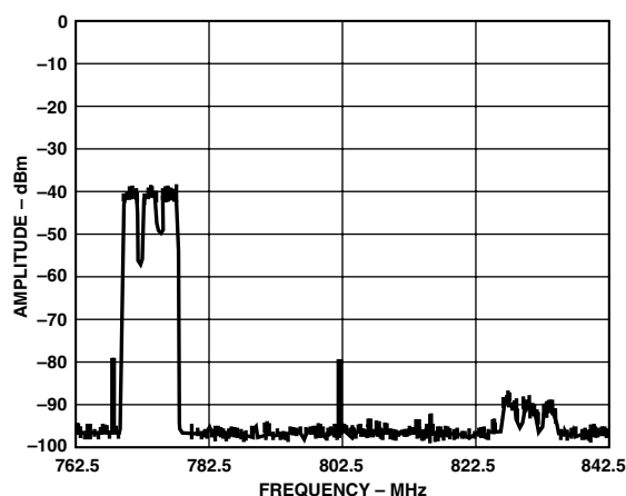
Figure 55. AD9777/AD8345 Synthesizing a Three-Carrier WCDMA Signal at an LO of 800 MHz
