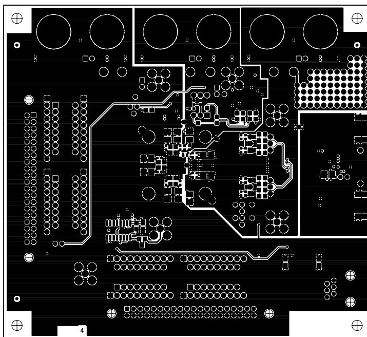
Figure 69. AD9777 Evaluation Board Layout, Layer Four (Bottom)
