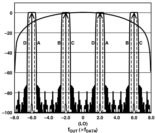
Figure 40. 8× Interpolation, Complex f_{DAC}/4 Modulation
