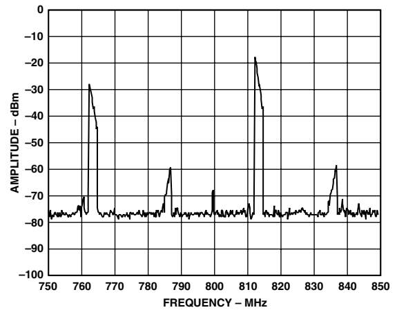
Figure 47. AD9777 Complex Output from Figure 46, Now Quadrature Modulated by AD8345 (LO = 800 MHz)
