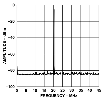
TPC 22. Two-Tone IMD Performance, f_{DATA} = 90 MSPS, Interpolation = 4×
