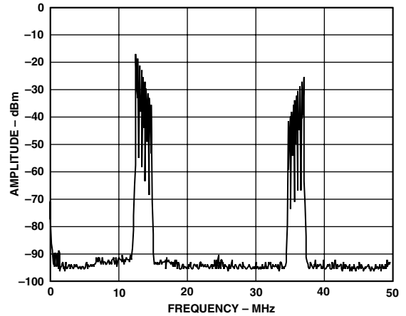
Figure 46. AD9777, Real DAC Output of Complex Input Signal Near Baseband (Positive Frequencies Only), Interpolation = 4x, Complex Modulation in AD9777 = +f_{DAC}/4
