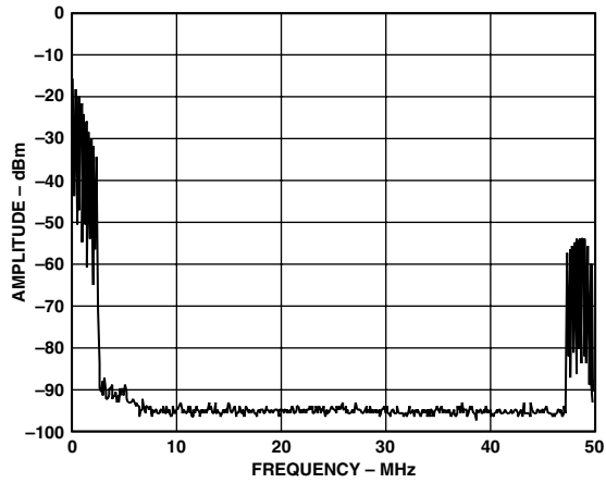
Figure 44. AD9777, Real DAC Output of Complex Input Signal Near Baseband (Positive Frequencies Only), Interpolation = 4x, No Modulation in AD9777
