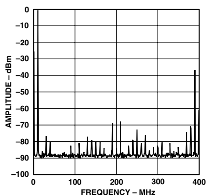
TPC 25. Single-Tone Spurious Performance, f_{OUT} = 10 MHz, f_{DATA} = 50 MSPS, Interpolation = 8×
