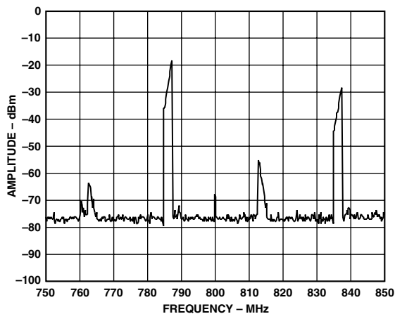
Figure 49. AD9777 Complex Output from Figure 48, Now Quadrature Modulated by AD8345 (LO = 800 MHz)
