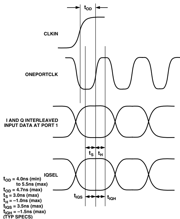
Figure 23. Timing Requirements in One Port Input Mode, with PLL Disabled
