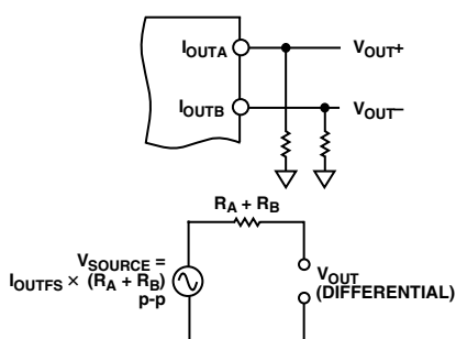
Figure 52. DAC Output Equivalent Circuit
