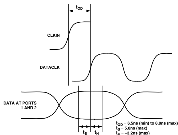
Figure 22. Timing Requirements in Two Port Input Mode, with PLL Disabled
