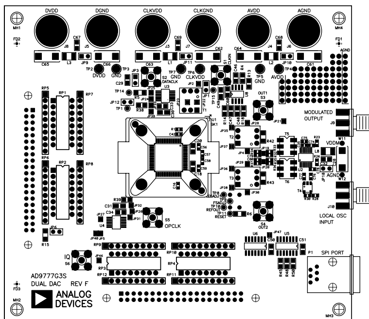
Figure 64. AD9777 Evaluation Board Components, Top Side
