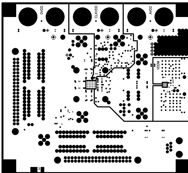
Figure 68. AD9777 Evaluation Board Layout, Layer Three (Power Plane)
