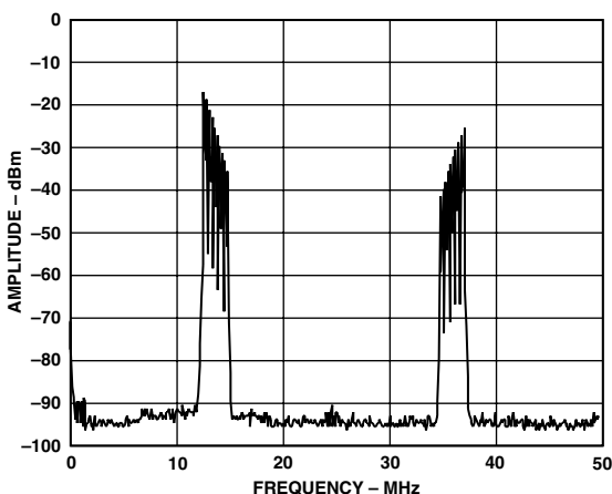
Figure 48. AD9777, Real DAC Output of Complex Input Signal Near Baseband (Negative Frequencies Only), Interpolation = 4\times , Complex Modulation in AD9777 = -f_{DAC}/4
