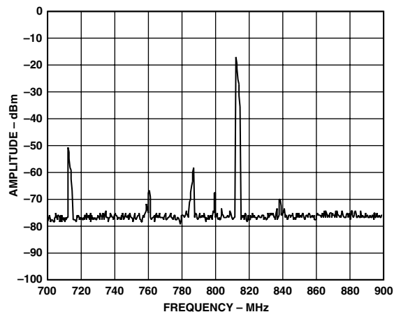
Figure 51. AD9777 Complex Output from Figure 50, Now Quadrature Modulated by AD8345 (LO = 800 MHz)
