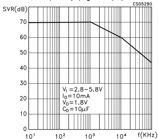
Figure 11. Supply voltage rejection vs. frequency ( C_o = 10 \mu F )
