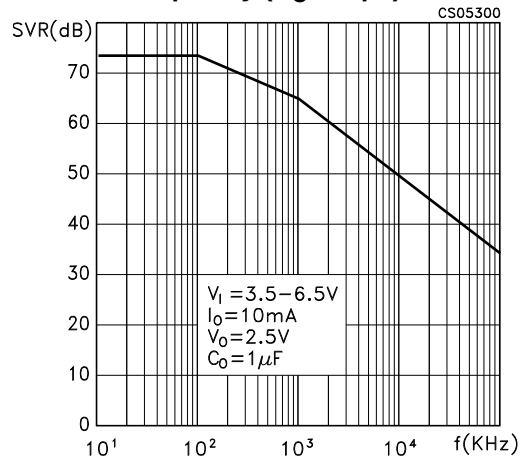
Figure 12. Supply voltage rejection vs. frequency ( C_o = 1 \mu F )
