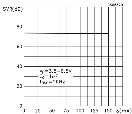
Figure 10. Supply voltage rejection vs. output current ( C_o = 1 \mu F )
