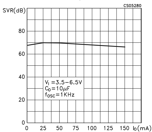
Figure 9. Supply voltage rejection vs. output current ( C_o = 10 \mu F )
