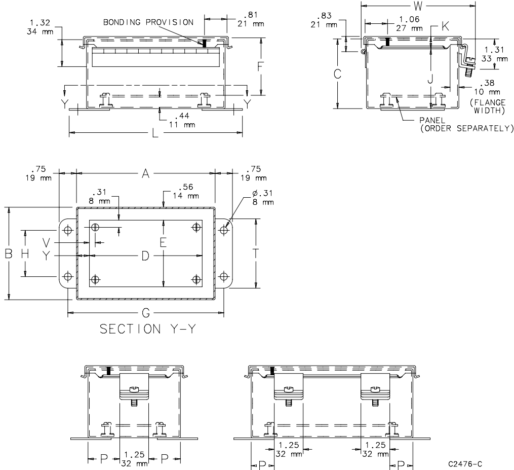
View showing clamp end of box when one clamp is used. View showing clamp end of box when two clamps are used. When A=8.00 (203mm) or more, use two clamps.
