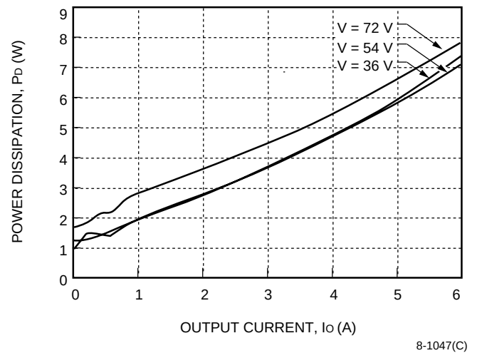
Figure 29. CW030A Power Dissipation vs. Output Current
