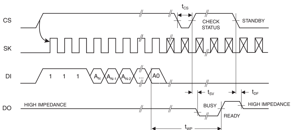
Figure 8. ERASE Timing
