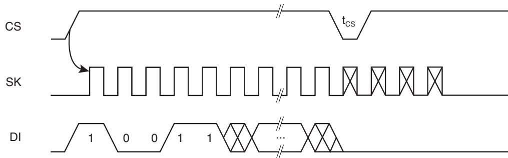
Figure 4. EWEN Timing (1)
