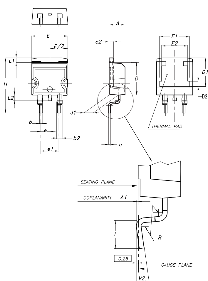
Figure 11. D 2 PAK package outline
