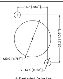
AC*MP
