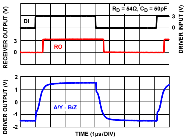
FIGURE 24. V_{CC} = 3.3V , DRIVER AND RECEIVER WAVEFORMS (ISL32430E, ISL32432E, ISL32437E)
