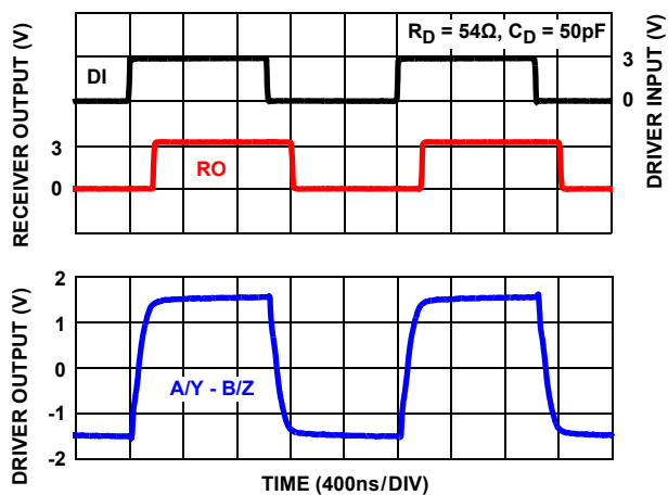
FIGURE 25. V_{CC} = 3.3V , DRIVER AND RECEIVER WAVEFORMS (ISL32433E, ISL32435E)
