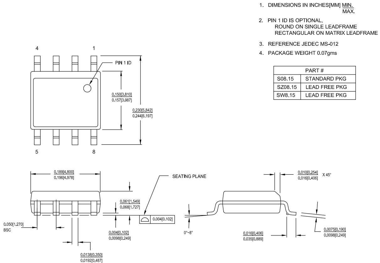
Figure 17. 8-pin SOIC (150 Mils) Package Outline, 51-85066
