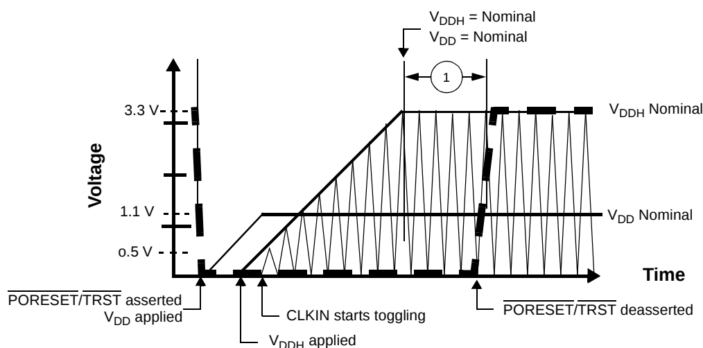
Figure 7. Start-Up Sequence: V_{\text{DD}} Raised Before V_{\text{DDH}} with \text{CLKIN} Started with V_{\text{DDH}}
