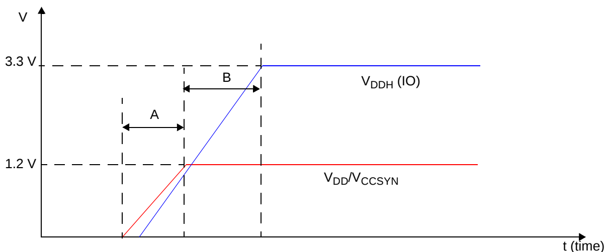
Figure 8. Power-Up Sequence for V_{\text{DDH}} and V_{\text{DD/VCCSYN}}
