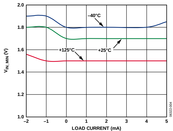
Figure 4. Minimum Input Voltage vs. Load Current, V_{OUT} = 0.5\text{ V}
