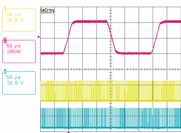
FIGURE 47. 2-PHASE CPU MODE V_{ID} ON THE FLY, 1.075V/0.875V , 2-PHASE CONFIGURATION, PSI\# = 1 , DPRSLPVR = 0 , Ch1: PHASE1, Ch2: V_0 , Ch3: PHASE2
