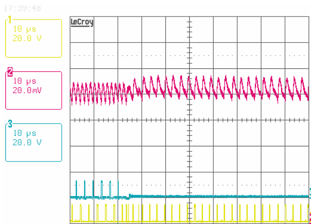
FIGURE 48. PHASE ADDING ( PSI\# TOGGLE), I_O = 15A , V_{ID} = 1.075V , Ch1: PHASE1, Ch2: V_0 , Ch3: PHASE2, Ch4: N/A
