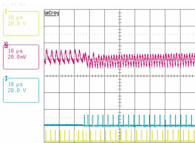
FIGURE 49. PHASE DROPPING ( PSI\# TOGGLE), I_O = 15A , V_{ID} = 1.075V , Ch1: PHASE1, Ch2: V_0 , Ch3: PHASE2, Ch4: N/A
