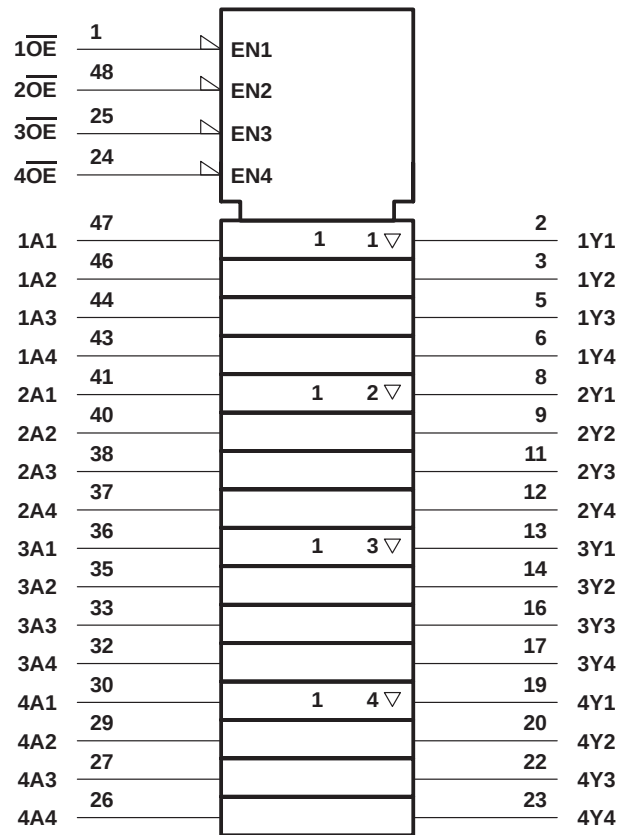
logic symbol†
