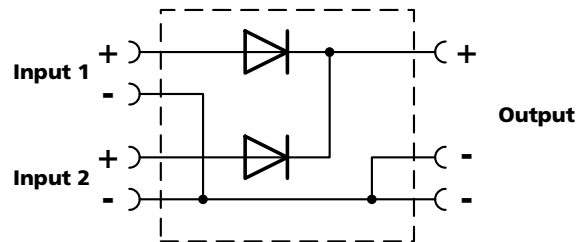
Fig. 7-1 Functional diagram
