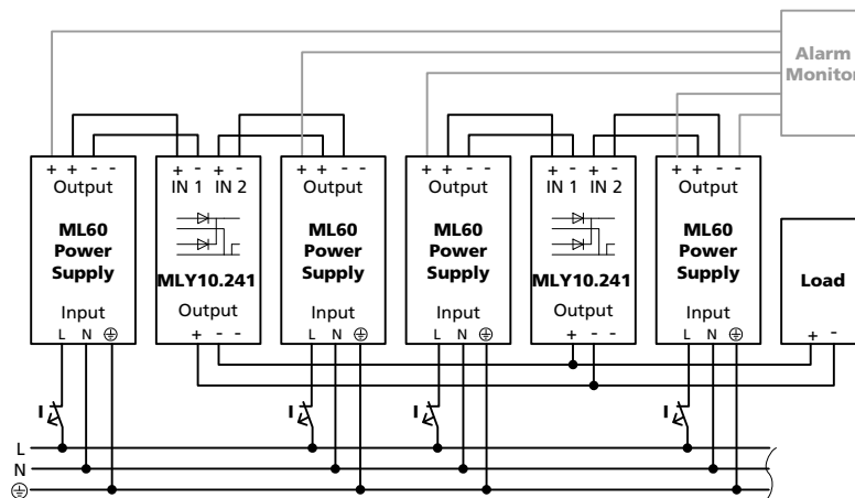
Fig. 18-2 Wiring diagram, N+1 Redundancy, 7.5A output current
