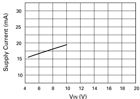
Supply Current v VIN N Phase Device
