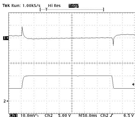
Fig.6a Line Regulation 0.5A load
