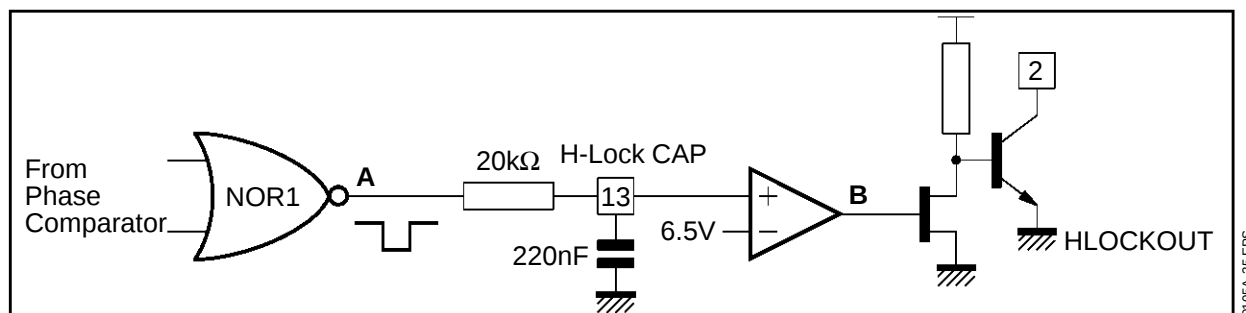
Figure 15 : LOCK/UNLOCK Block Diagram
