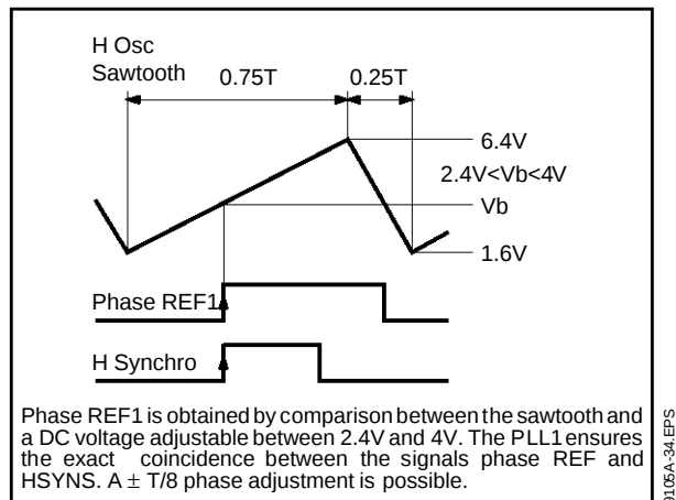
Figure 14 : PLL1 Timing Diagram
