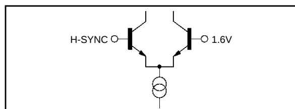
Figure 9 : Input Structure
