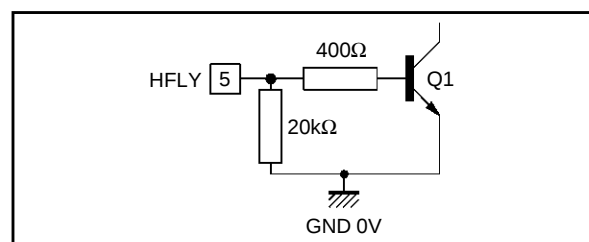
Figure 17 : Flyback Input Electrical Diagram
