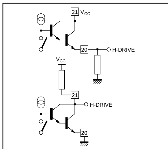
Figure 19 : Output stage simplified diagram, showing the two possibilities of connection
