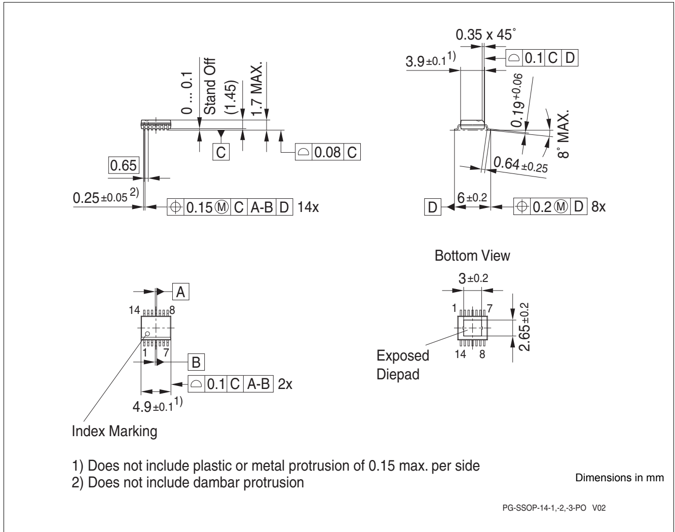
Figure 27 PG-SSOP14
