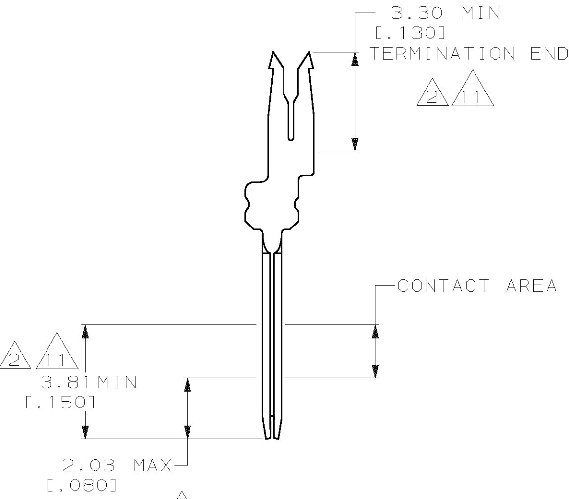
DETAIL M SCALE 8:1 TYPICAL
