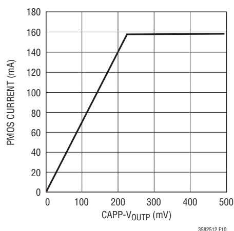
Figure 9. PMOS Current vs Voltage During Normal Operation
