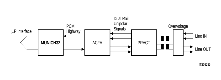
Figure 87 ISDN Interface
