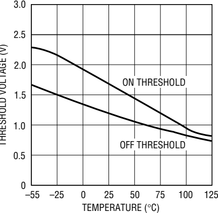
On/Off Thresholds
