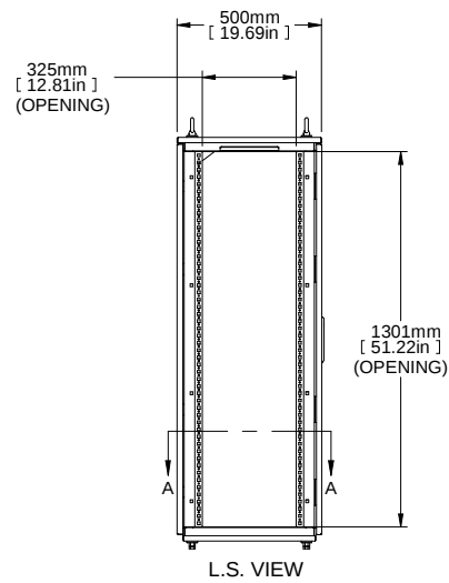
L.S. VIEW
