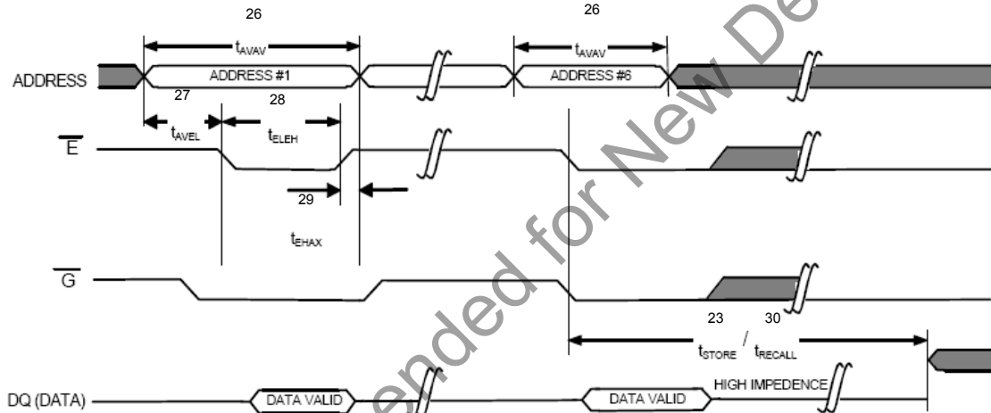
Figure 11. Software STORE/RECALL CYCLE: \overline{E} Controlled [13]
