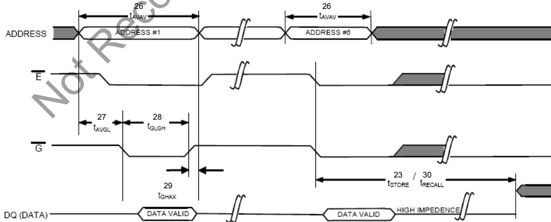
Figure 12. Software STORE/RECALL CYCLE: \overline{G} Controlled [13]
