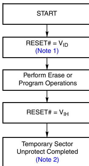
Figure 7.1 Temporary Sector Unprotect Operation
