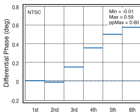
Figure 14. Differential Phase, V_{OUT}
