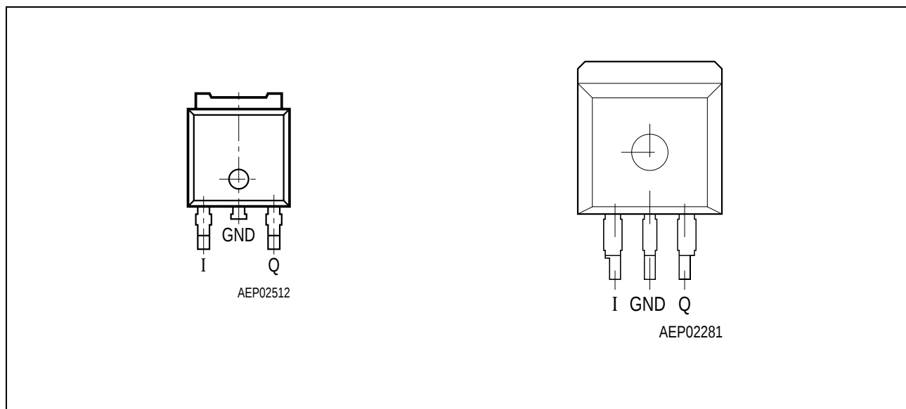
Figure 2 Pin Configuration P-T0252-3 (D-PAK), P-T0263-3 (D 2 -PAK)(top view)
