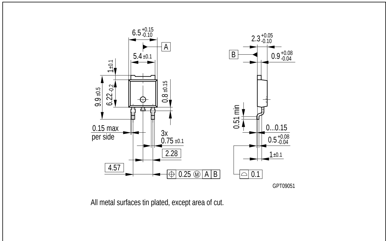
Figure 4 P-T0252-3-1 (Plastic Transistor Single Outline)
