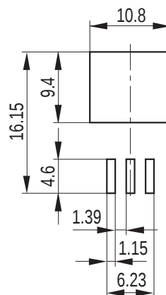
Figure 8 Foot Print for P-TO263-3-1 (Plastic Transistor Single Outline)
