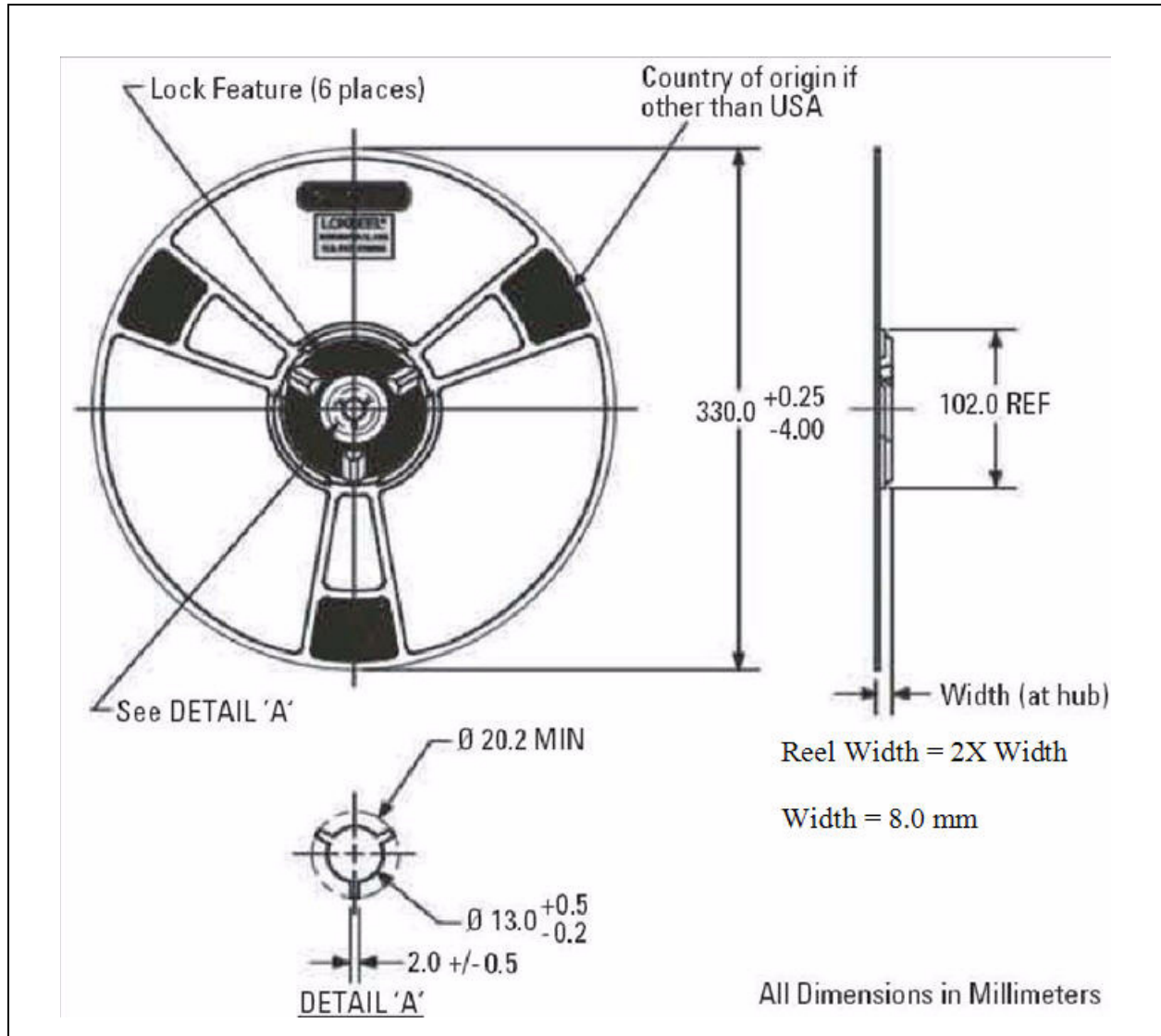
Figure 9.3 Reel Dimensions
