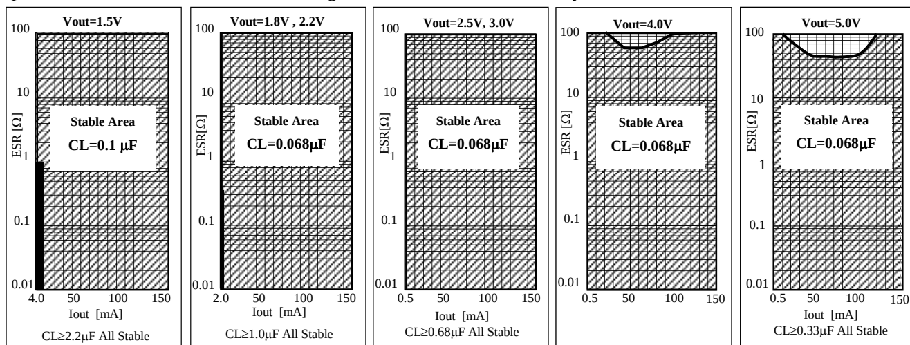
Figure 2. Output voltage, Output current vs. Stable Operation Area
